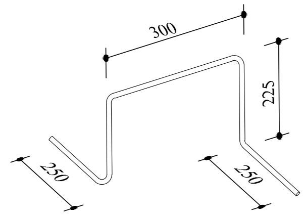
467T12-32@1000x1000 CHAIR FOR 300 MM SLAB THICKNESS
