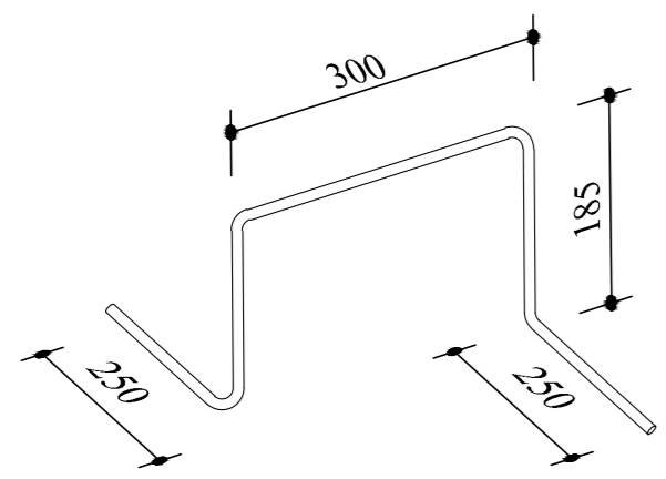
1744T12-31@1000X1000 CHAIR FOR 260 MM SLAB THICKNESS
